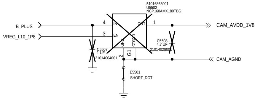
ANALOG REGULATOR 1.8V
