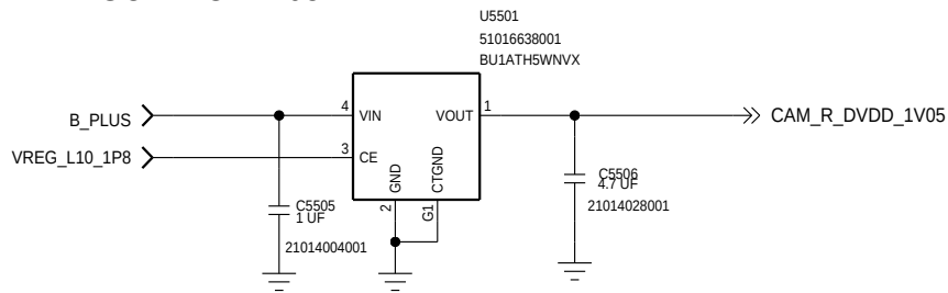
DIGITAL REGULATOR 1.05V
